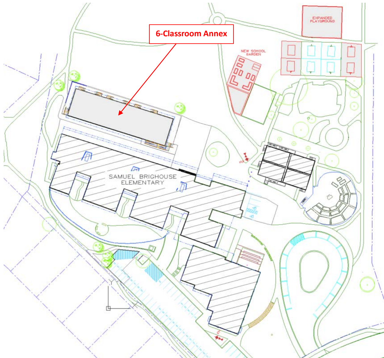
Project Site Plan - Samuel Brighthouse Elementary Annex
